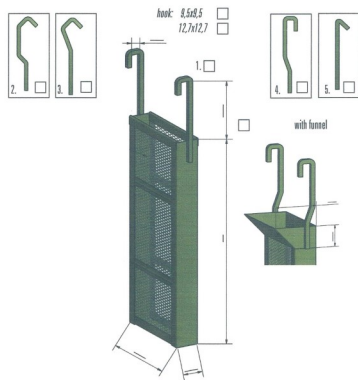
Titanium Fine Mesh Anode Basket
