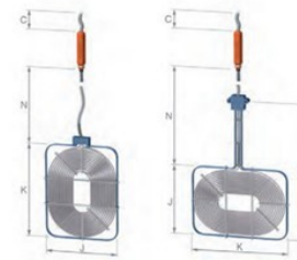
Pancake Style Heater
